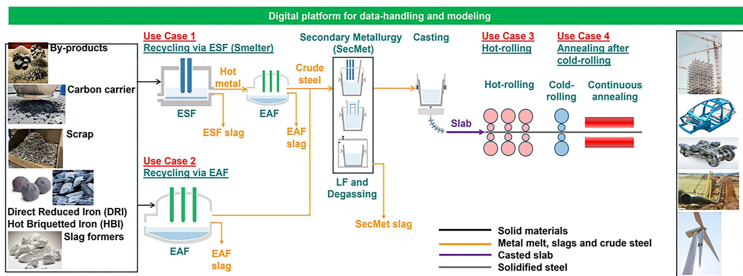
Figure 1. CircSmeltSteel concept covering both the upstream and the downstream processes.
